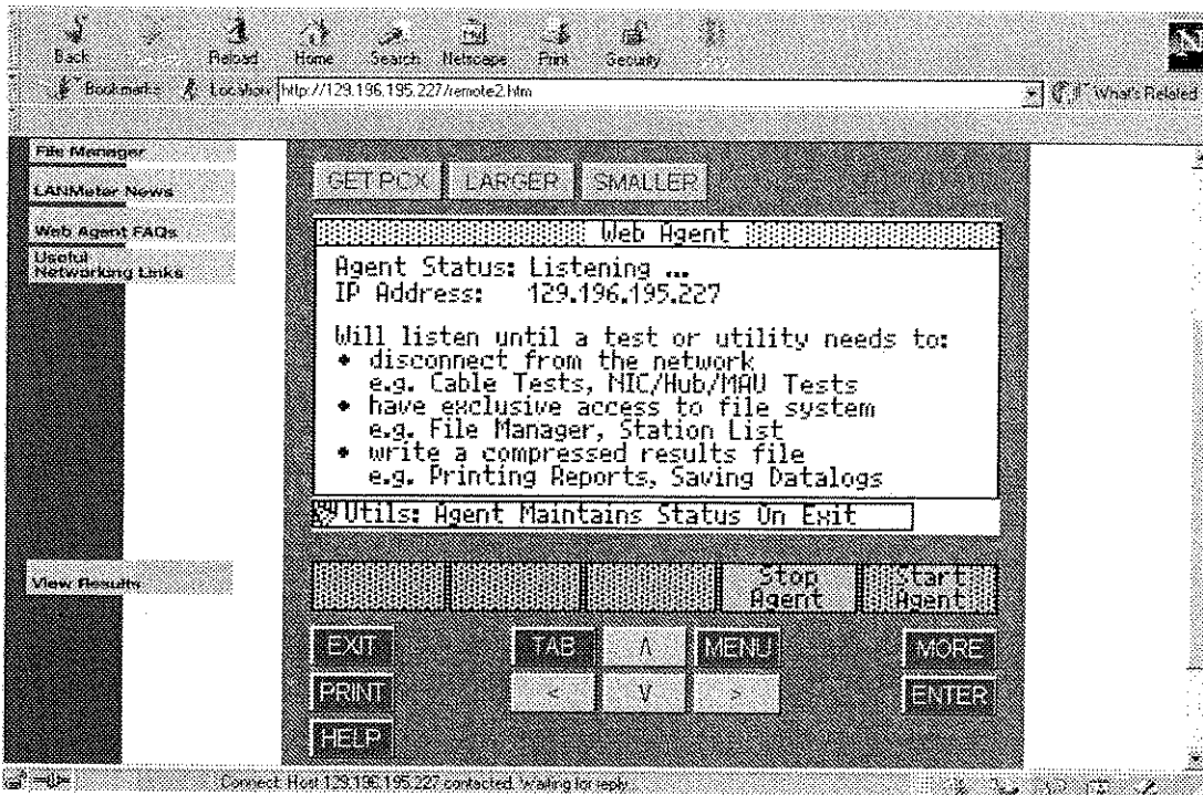
Figure 13-10. WebRemote Control
